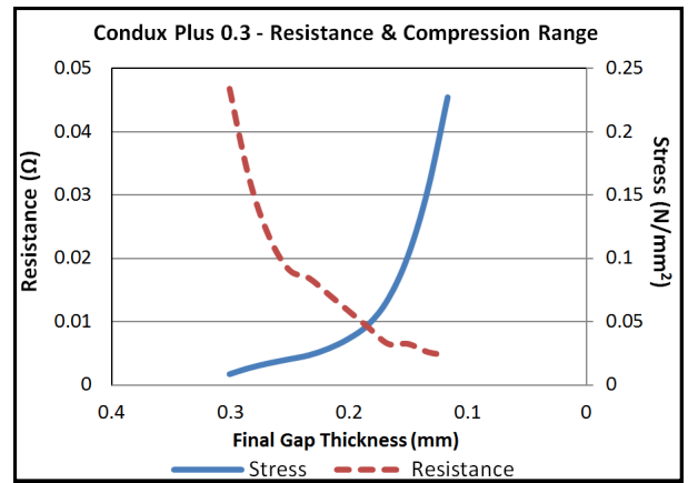
Figure 1: Condux Plus 0.3 mm Resistance & Compression
