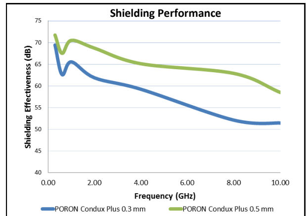
Figure 3: Condux Plus 0.3 mm & 0.5 mm Shielding Effectiveness Graph
