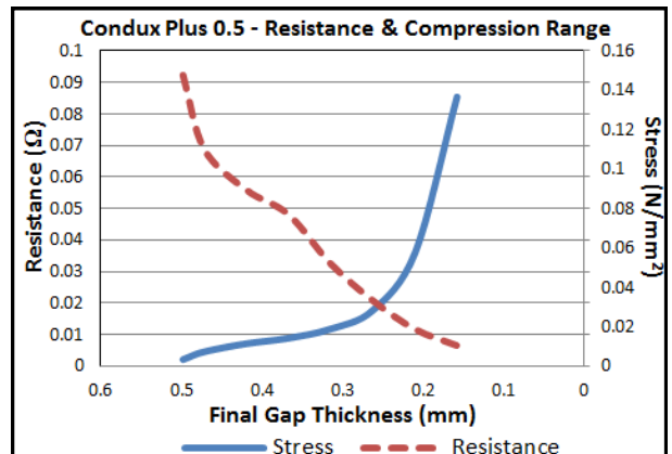
Figure 2: Condux Plus 0.5 mm Resistance & Compression
